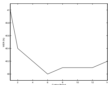
Fig. 2. Performance of Periodic Lattice Cutting with different cutting periods for A^* SMBR decoding on the swbd2-98 test set
