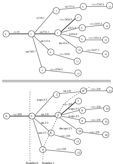
Fig. 1. (top) A word lattice \mathcal{W} and (bottom) its acceptor \hat{A} showing the Levenshtein alignment between W \in \mathcal{W} and \tilde{W} (shown as the path in bold).
